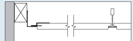
6. Shadow batten, angle trim and edge clips
