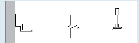
4. Shadow moulding
